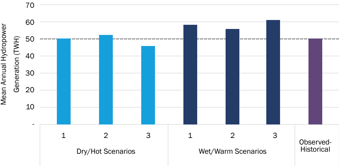
Figure 3.9. Mean annual hydropower generation (TWh)
