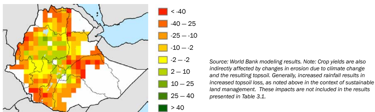
Figure 3.4. Yield changes for teff, 2001–2020 to 2041–2060 under climate change
