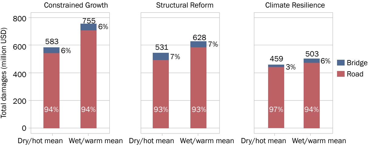
Figure 3.10. Annual roads and bridges costs, 2041–2050
