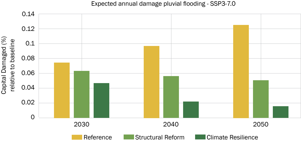
Figure 3.12. Capital damages to Addis Ababa, SSP3-7.0
